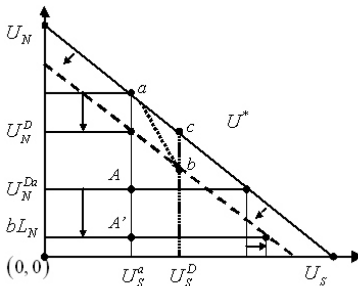
Figure 2: Strategic Destruction as a Bargaining Ploy
